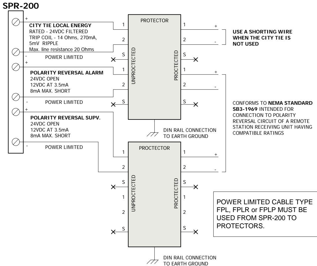
Figure 2: Polarity reversal and city tie module terminal connection
