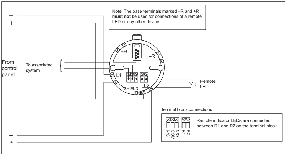
Fig 1 Summit Low Power Relay Base wiring diagram
